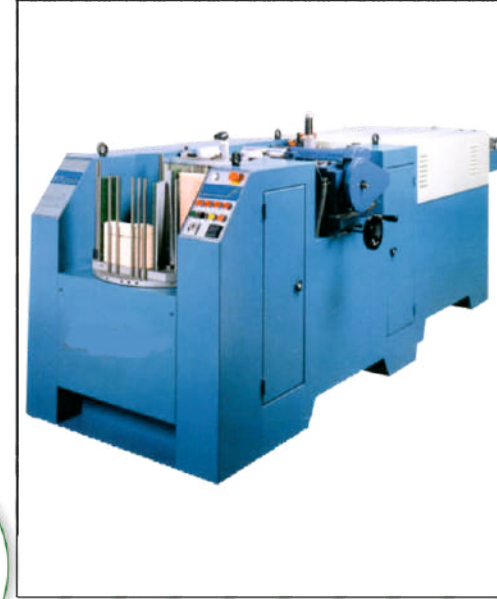
İLAÇ SÜRME + KURUTMA AUTOMATIC INSOLE CEMENTING AND DRYING
